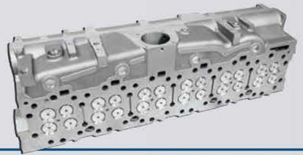
CYLINDER HEAD FOR CATERPILLAR C15 22012100002
